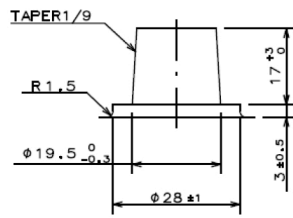
POS TERMINAL
