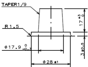
NEG TERMINAL
